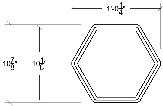
Plan view SCALE: 1-1/2"=1'-0"
